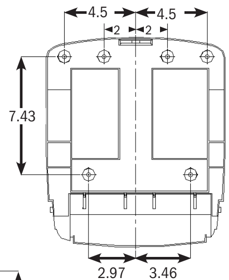
BACK (inches)
