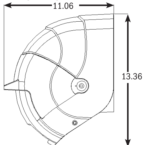
SIDE (inches)
