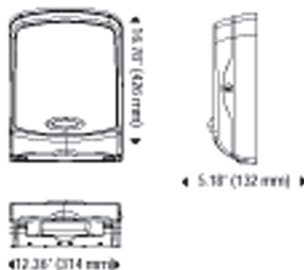
Dispenser Dimensions
