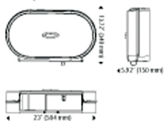
Dispenser Dimensions
